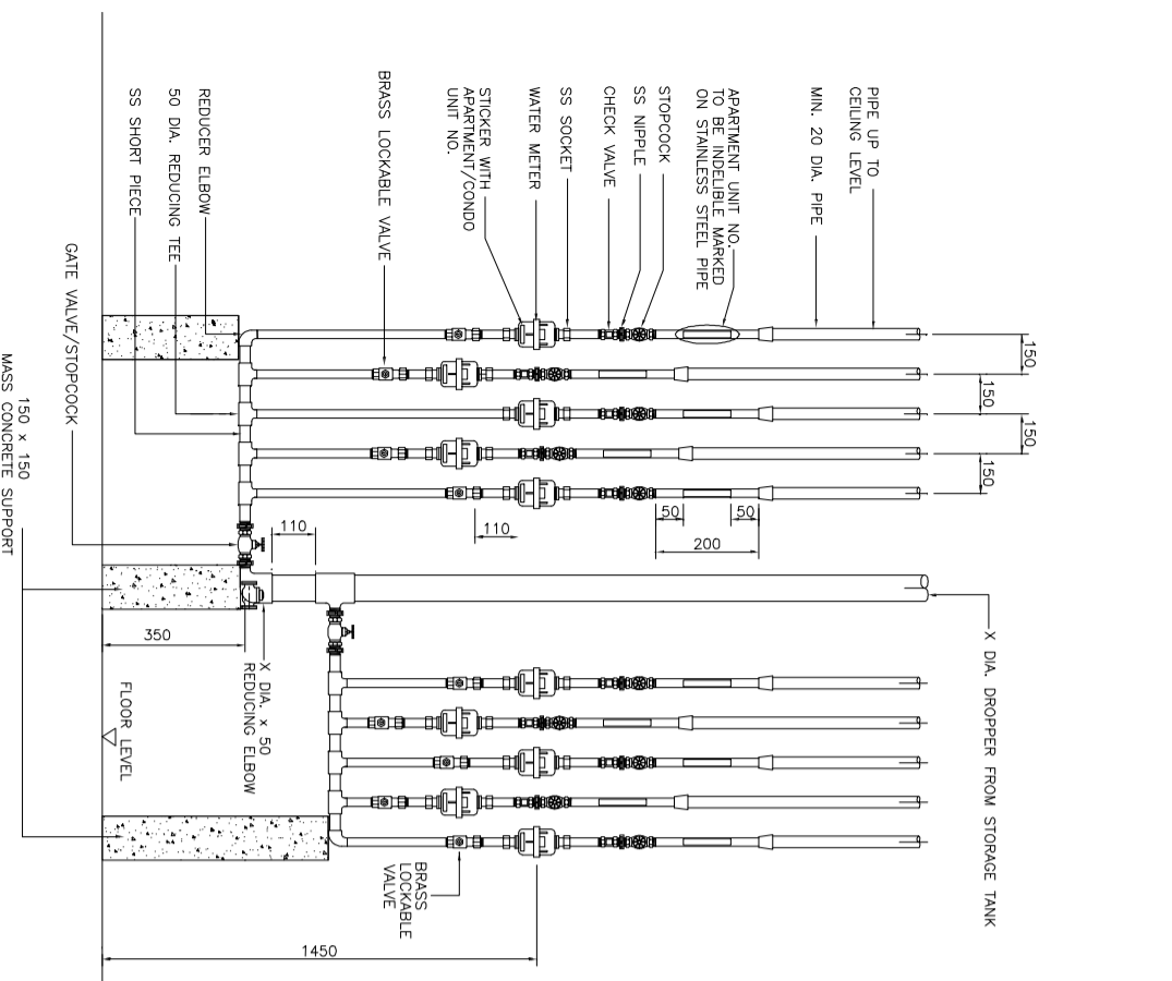
DETAIL OF METERSTAND INSTALLED IN VERTICAL FOR HIGH RISE APARTMENT/CONDOMINIUM
