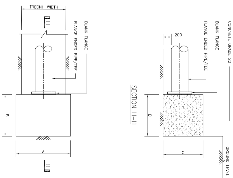
DETAILS OF THRUST BLOCK FOR BLANK FLANGE
