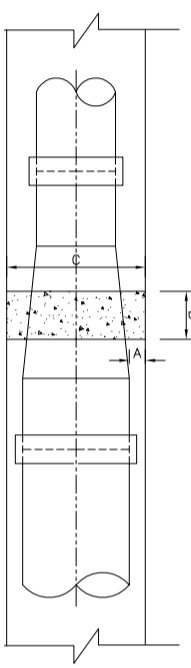
DETAILS OF THRUST BLOCK FOR TAPER
