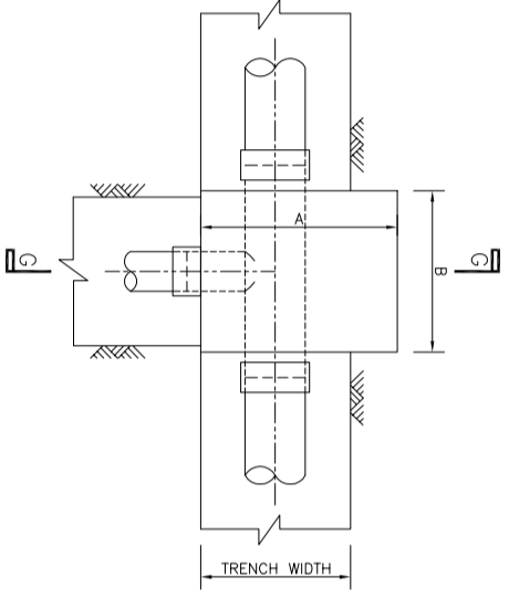
DETAILS OF THRUST BLOCK FOR TEE
